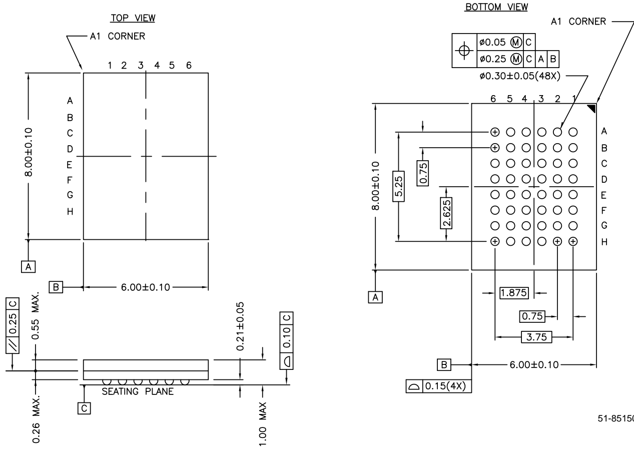
Figure 6. 48-pin VFBGA (6 × 8 × 1 mm) BV48/BZ48, 51-85150
