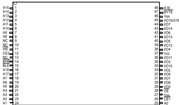
Figure 3. 48-pin TSOP I (512 K x 16/1 M x 8) (Top View) [1, 3]
