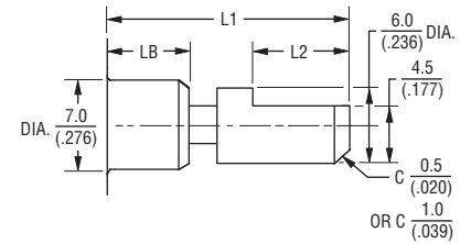
FLATTED SHAFT
