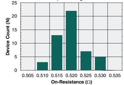
Typical On-Resistance Distribution (N=50, I_F=1\text{mA} , I_L=400\text{mA} )
