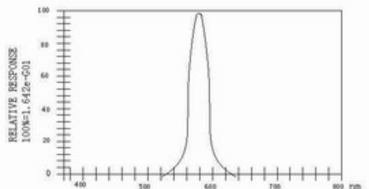
Luminous Spectrum (Ta=25°C) SPECTRAL RADIANCE
