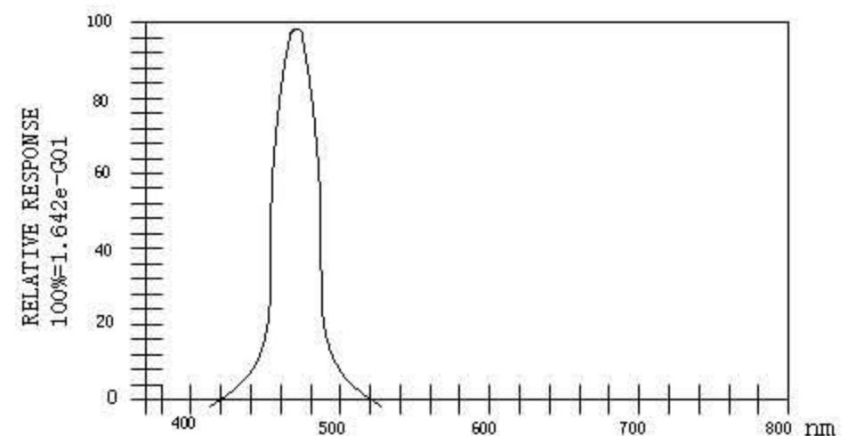
Luminous Spectrum (Ta=25°C) SPECTRAL RADIANCE
